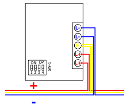
ML - 1410 AKILLI ADRESLİ SİSTEM SİREN
